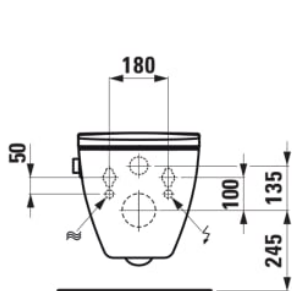
Connection with Laufen installation system LIS CW2
