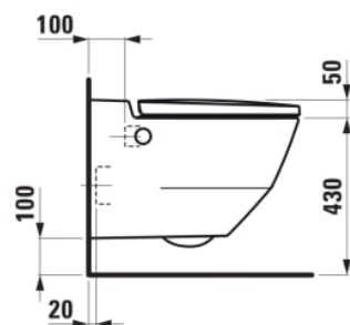
Connection with commercially available installation systems
