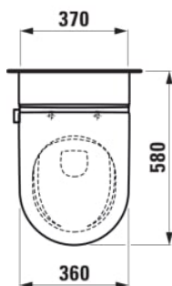
Connection with Laufen installation system LIS CW2
