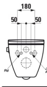
Connection with commercially available installation systems
